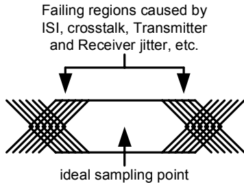
Figure 5. Sample Eye Diagram Over 1 UI
