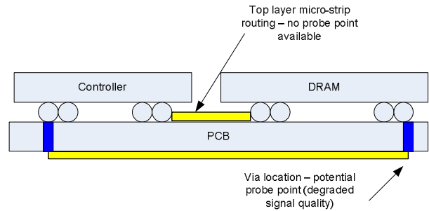
Figure 1. Micro-strip routing between two BGA devices
