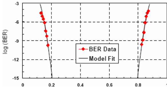
Figure 7. Measured System Jitter and Double Delta Model Fit at 6.4Gbps (DJ=23.3ps, RJ=2.62ps)
