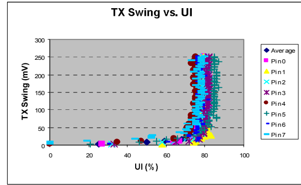
Figure 8. Transmitter swing vs. UI plot
