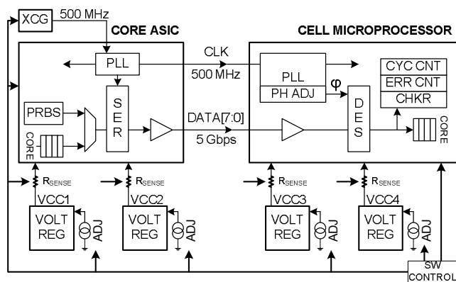
Figure 4. Assembled Measurement System for First Generation Systems Using FlexIO Technology
